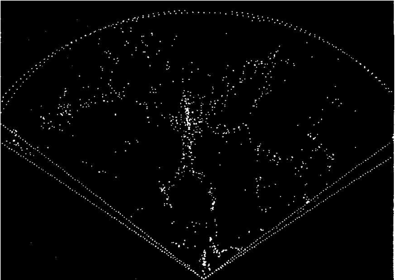
Fig. I1. A three-dimensional map showing a wedge of the Universe . This map was prepared at the Centre for Astrophysics, Harvard College Observatory and Smithsonian Astrophysical Observatory, by Margaret J. Geller, John P. Huchra and Valérie de Lapparent. It was published in Scientific American , March 1986 (Vol. 254, Number 3), page 49. The map reveals a cluster of galaxies which takes the apparent shape of a human figure. This human shape may gain special significance with the Concept of Dipolar Gravity stating that our universe is composed of two parallel worlds of a physical nature (i.e. the world of matter and the counter-world), which exactly copy each other like an object and its mirror reflection. The non-material one of these two worlds (i.e. the counter-world) is made of a substance (counter-matter) that is able to think in its natural constitution. This thinking substance forms the universal computer (UC) described in subsection I3.2, whose shape and dimensions must reflect the shape of our universe, and whose capabilities correspond to those of God. This in turn invokes a question as to whether the above human shape is a pure coincidence or astronomic confirmation to the biblical statement that "God created man in his own image".
